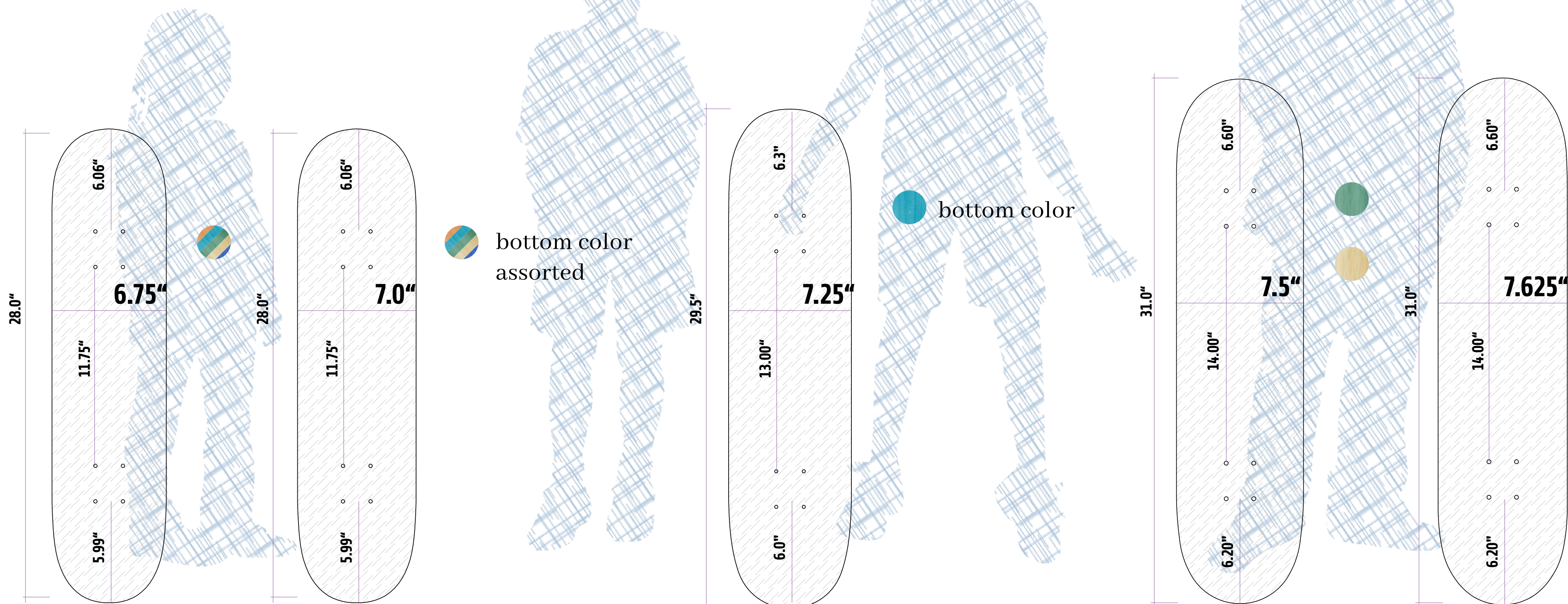
revised deck dimensions
